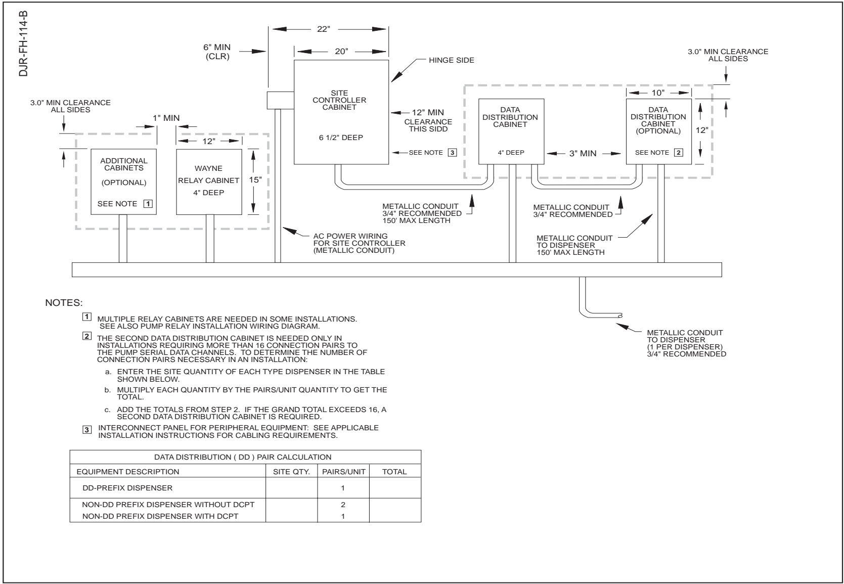
Figure D-1 Backroom Installation - Wayne Management Control System.
