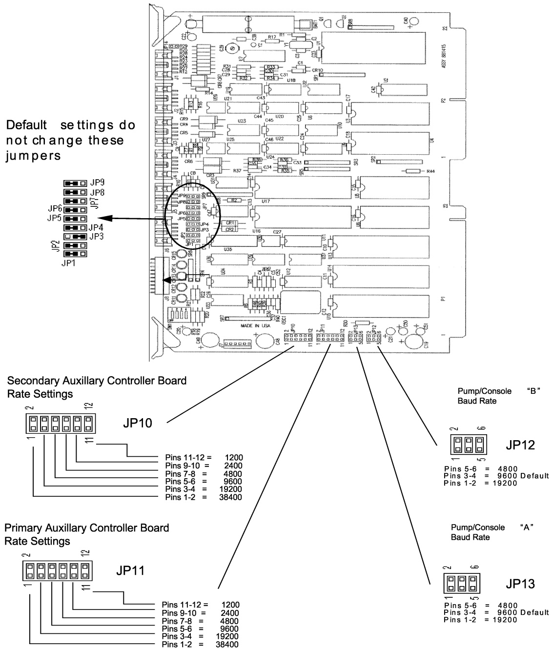
Figure 2-1 HyperPIB Board Jumper Settings
