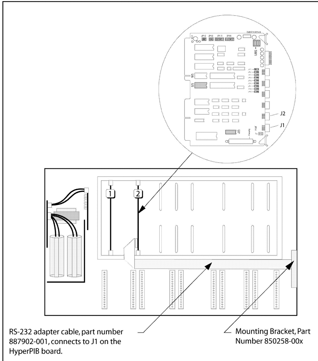
Figure 2-2 HyperPIB Board And RS-232 Installation
