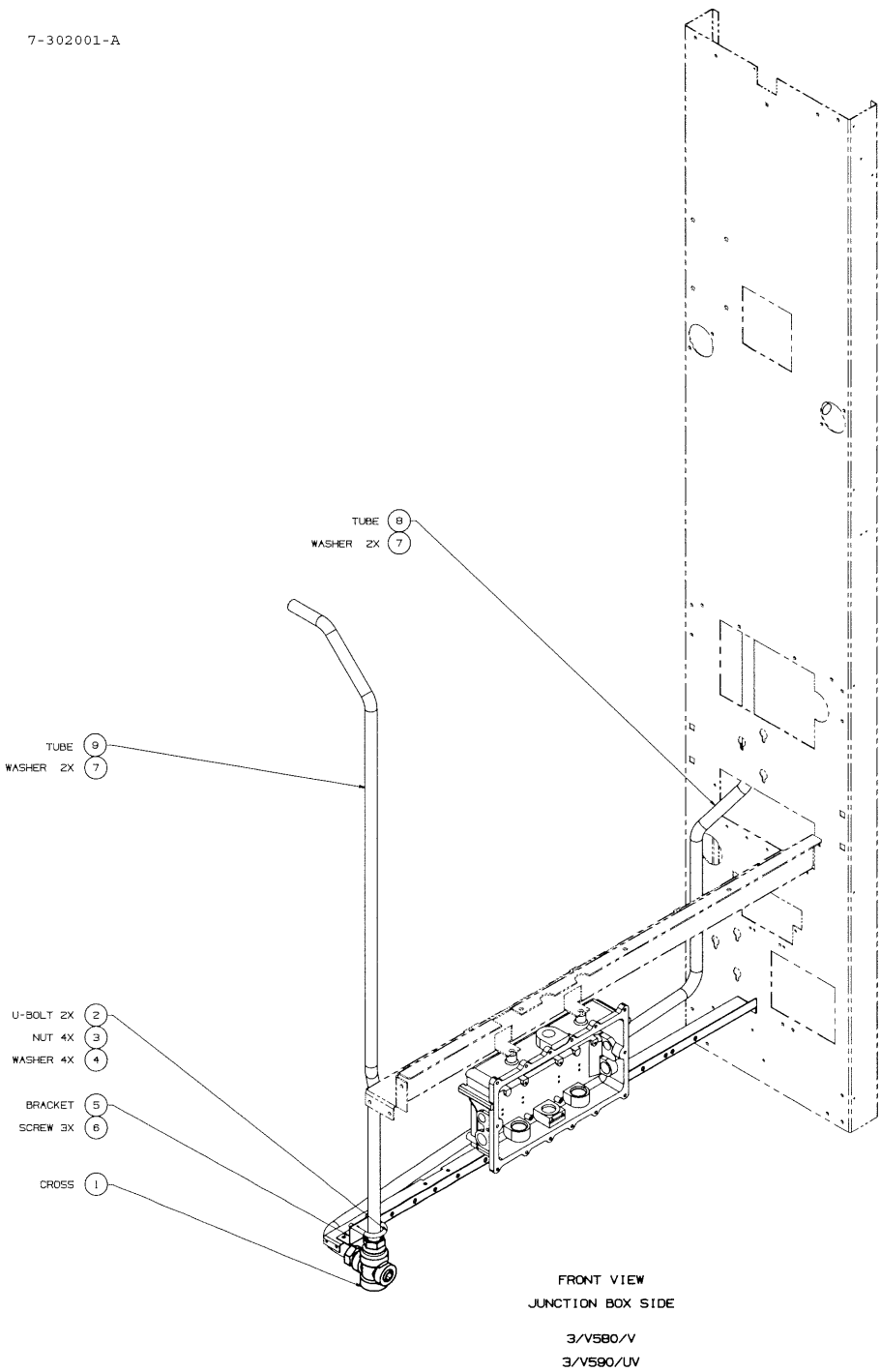
FIGURE 25. 7-302001-DWG - BALANCE VAPOR RECOVERY MODULE
