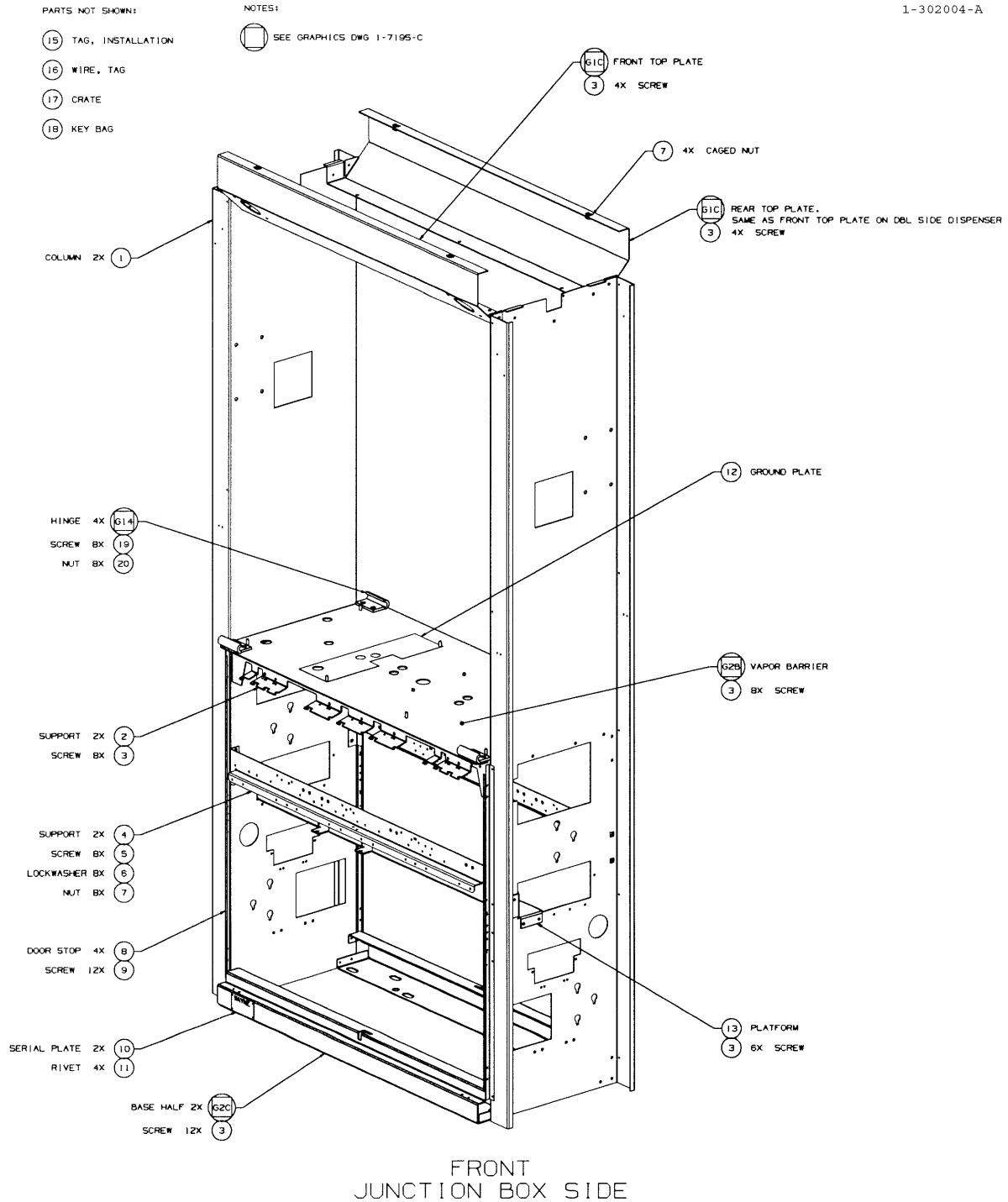
FIGURE 3. 1-302004-DWG - FRAME MODULE 3/V
