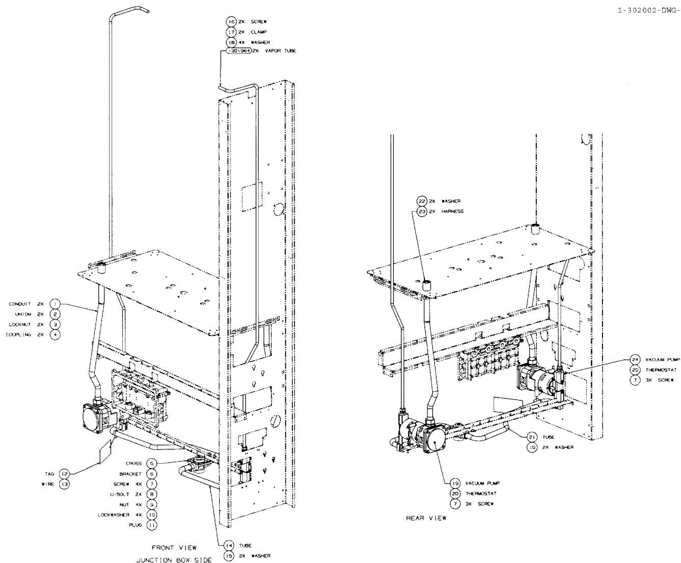
FIGURE 30. 1-302002-DWG - WAYNE VAC VAPOR RECOVERY MODULE
