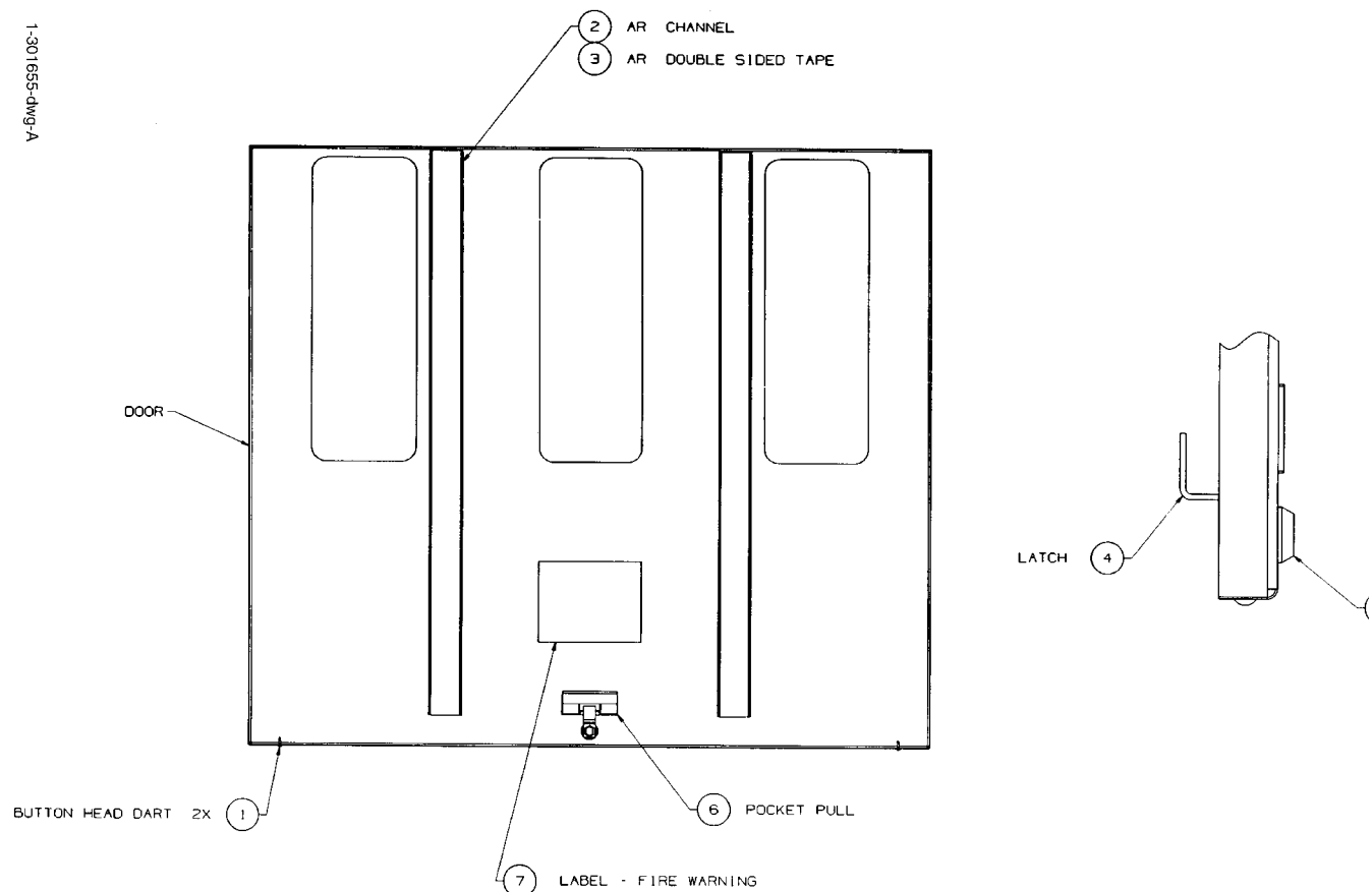
FIGURE 6. 1-301655-DWG - DOOR MODULE 3/V, ONE PIECE WIDE
