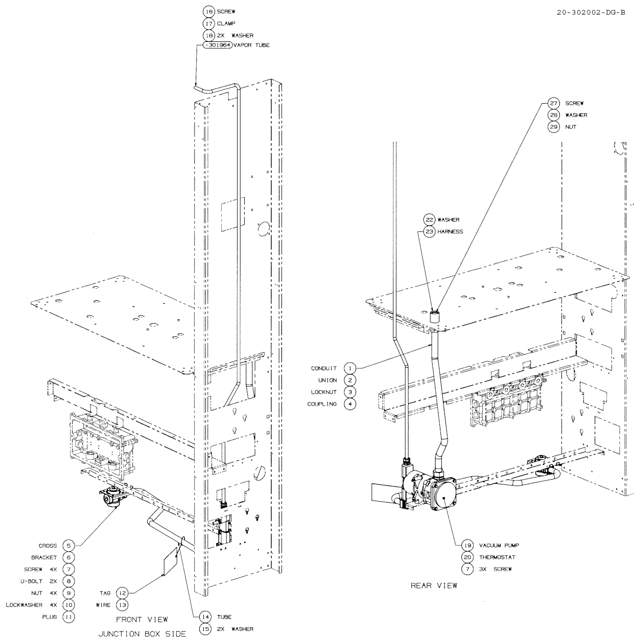
FIGURE 37. 20-302002-DWG - WAYNE VAC VAPOR RECOVERY MODULE
