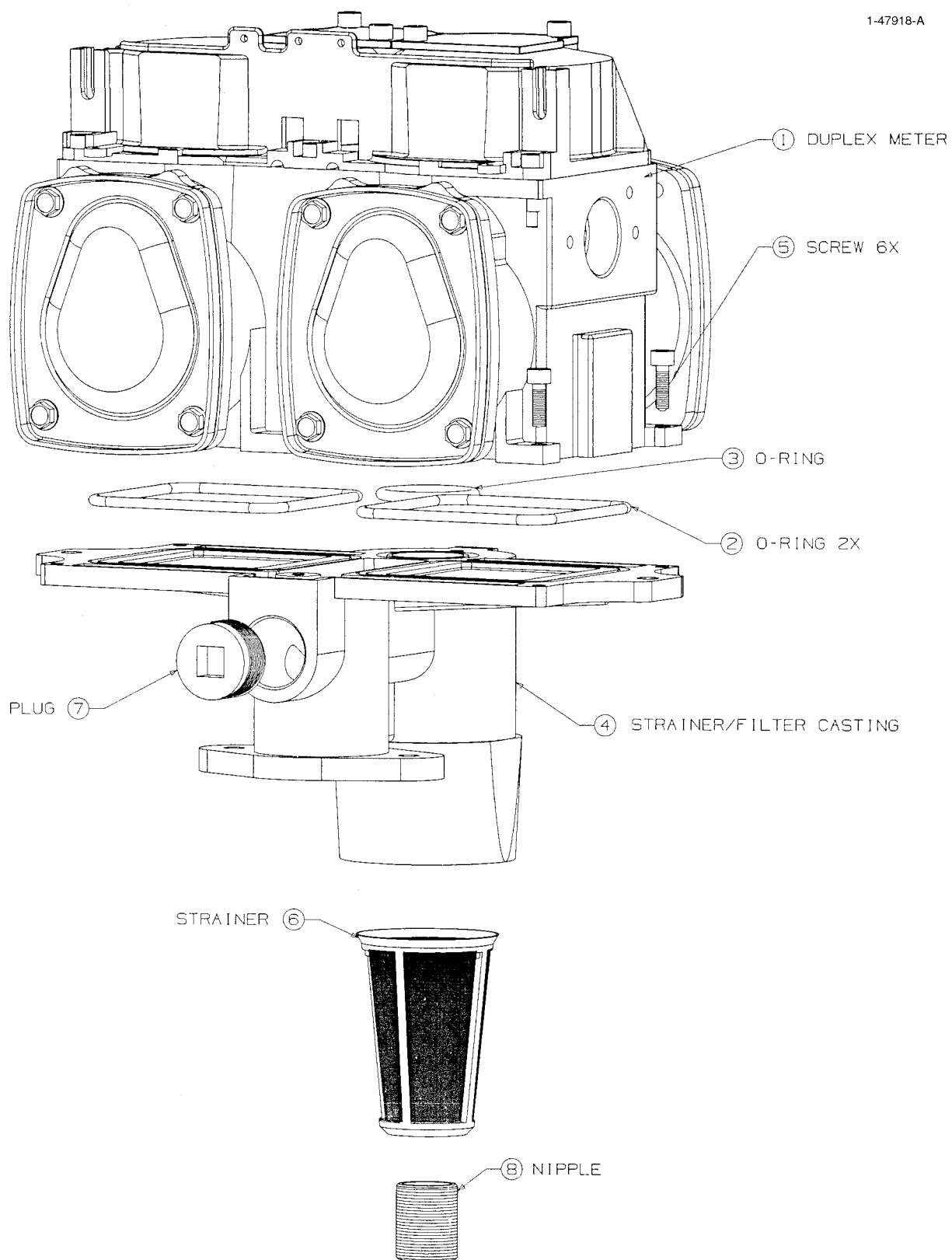
FIGURE 21. 1-47918-DWG - IMETER MODULE, 3/V REMOTE, SINGLE SIDED
