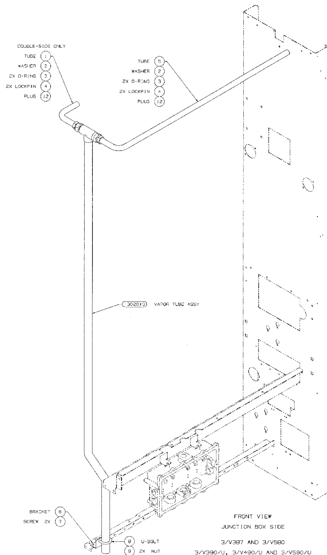
FIGURE 24. 1-302001-DWG - BALANCE VAPOR RECOVERY MODULE
