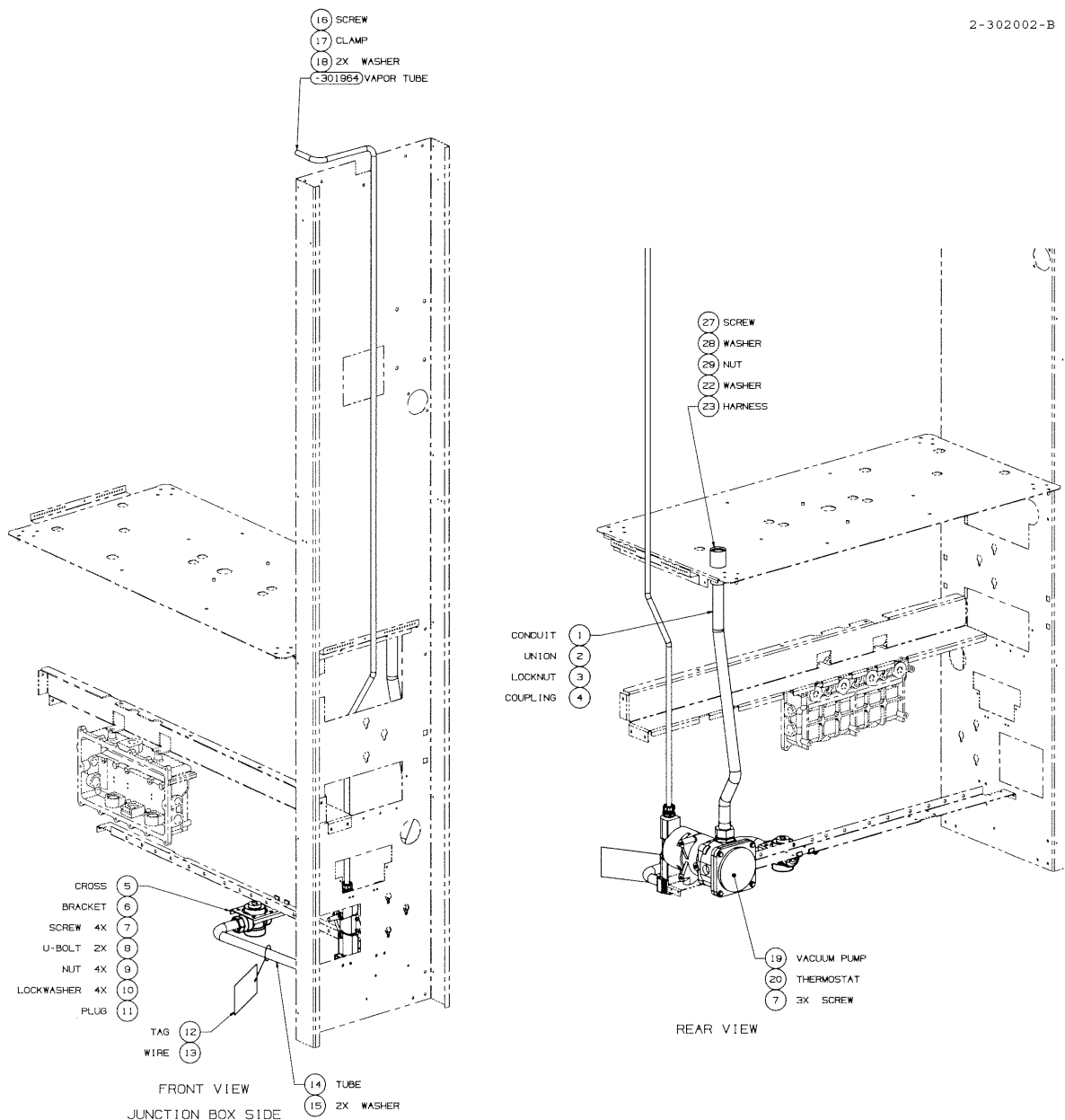
FIGURE 31. 2-302002-DWG - WAYNE VAC VAPOR RECOVERY MODULE
