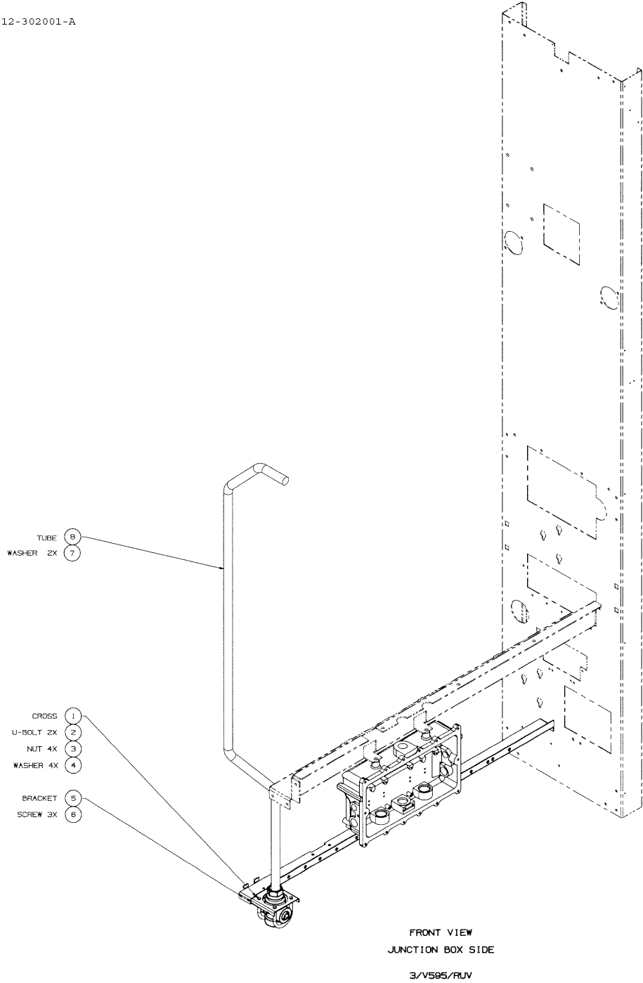
FIGURE 28. 12-302001-DWG - BALANCE VAPOR RECOVERY MODULE
