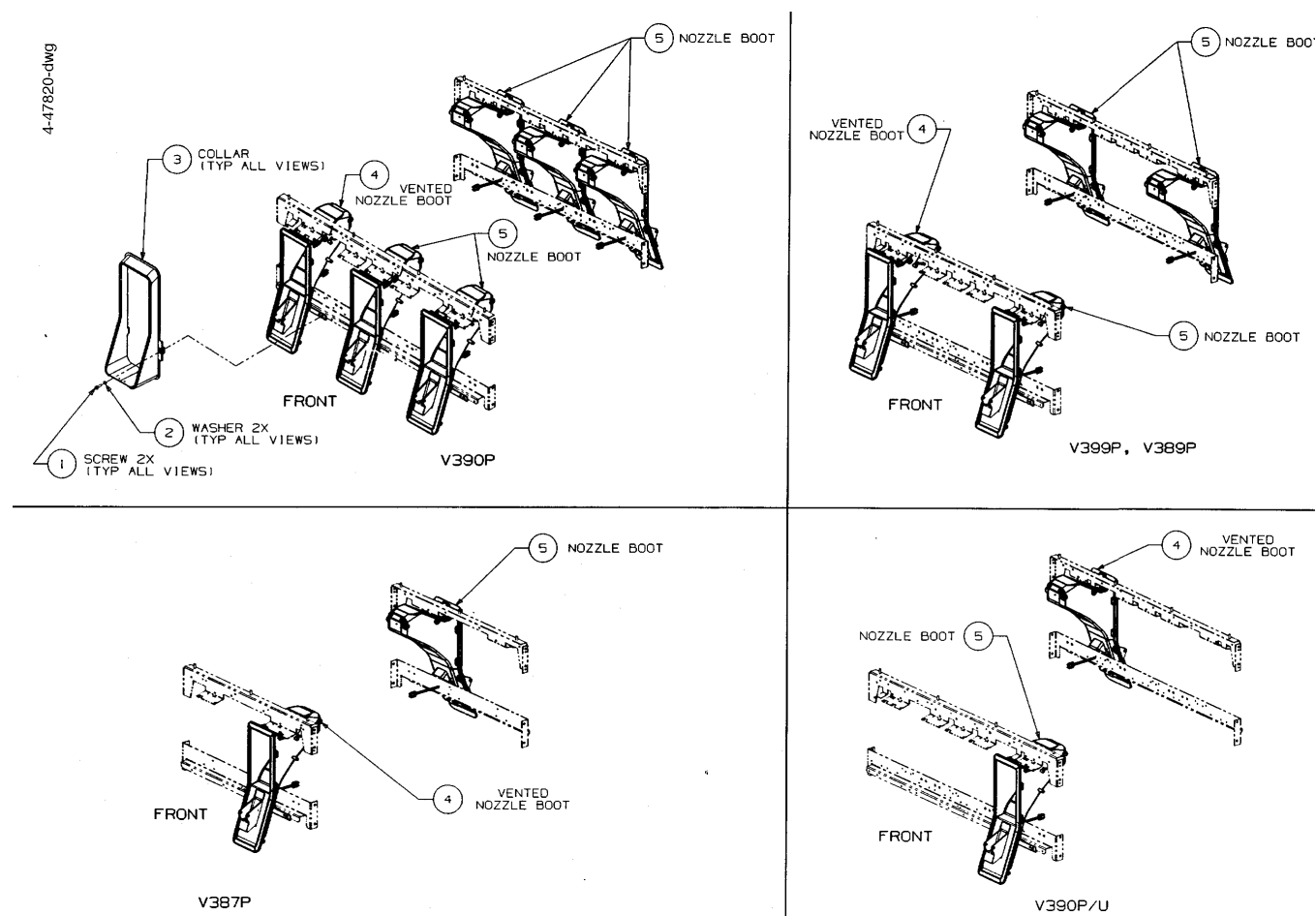
FIGURE 39. 4-47820-DWG - NOZZLE BOOT SUCTION
