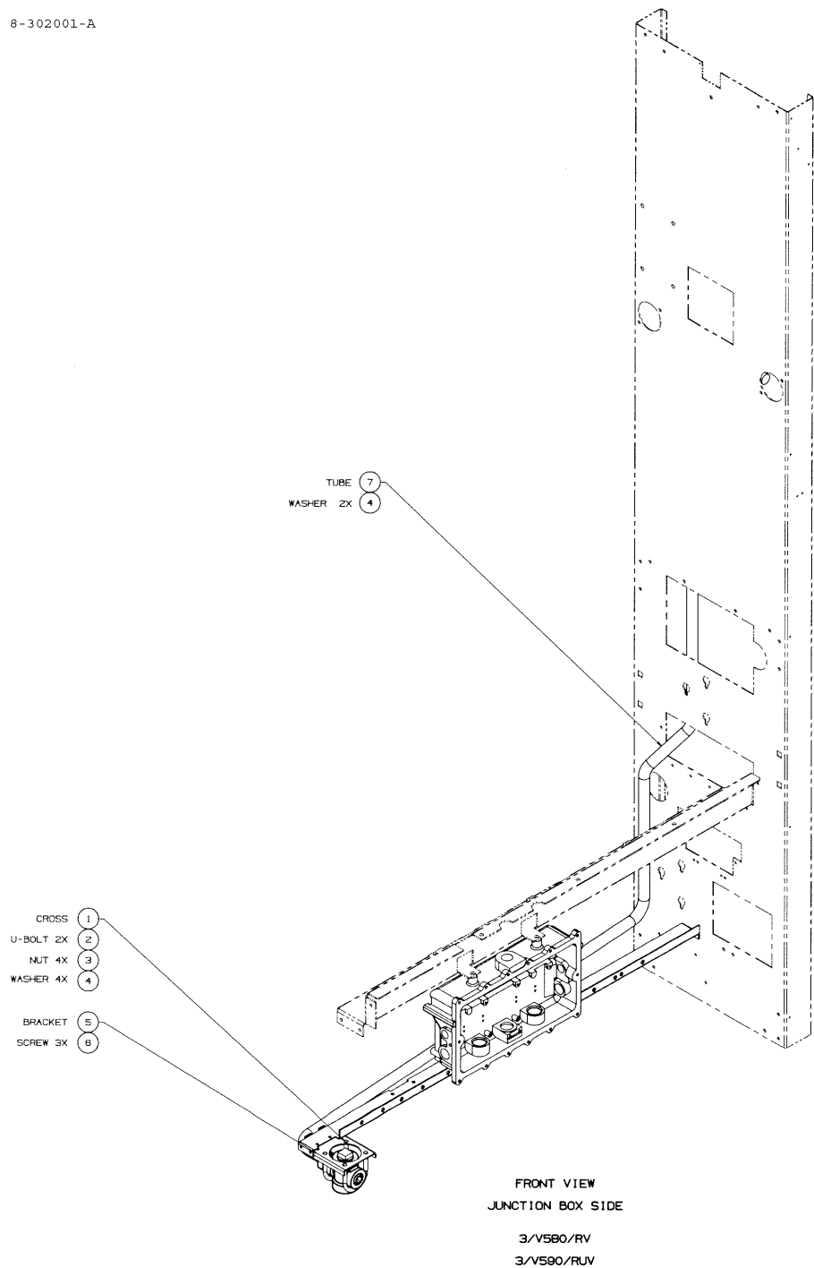
FIGURE 26. 8-302001-DWG - BALANCE VAPOR RECOVERY MODULE
