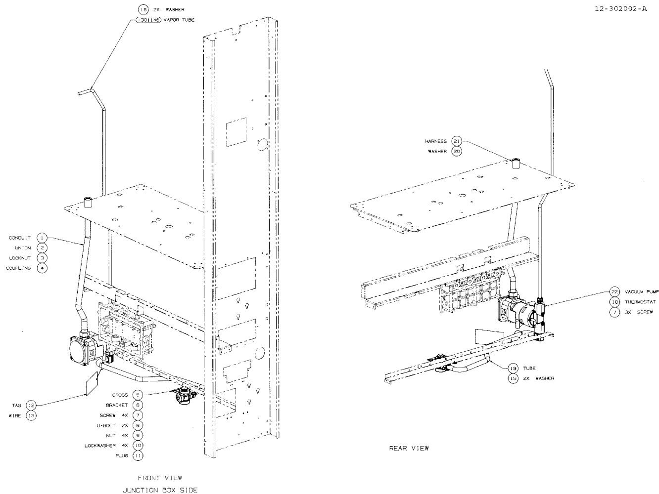
FIGURE 35. 12-302002-DWG - WAYNE VAC VAPOR RECOVERY MODULE
