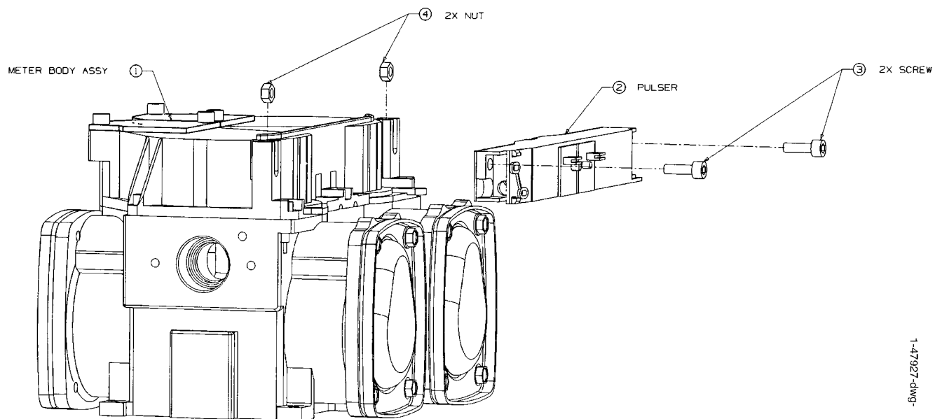
FIGURE 23. 1-47927-DWG - IMETER/PULSER ASSY
