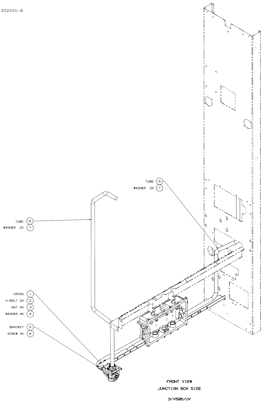
FIGURE 27. 11-302001-DWG - BALANCE VAPOR RECOVERY MODULE
