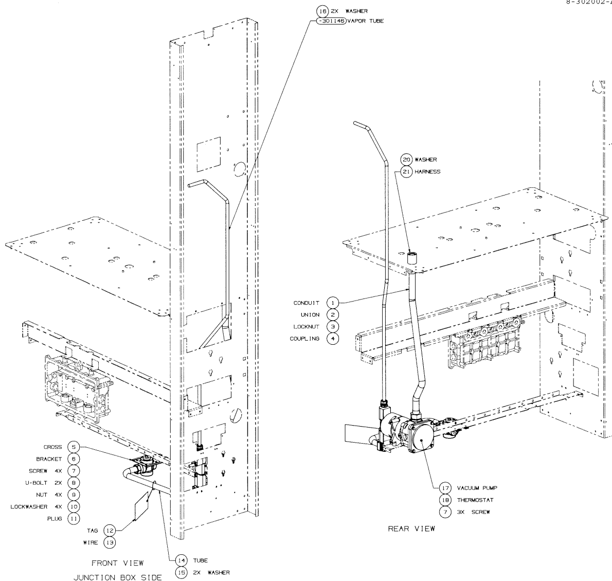
FIGURE 34. 8-302002-DWG - WAYNE VAC VAPOR RECOVERY MODULE
