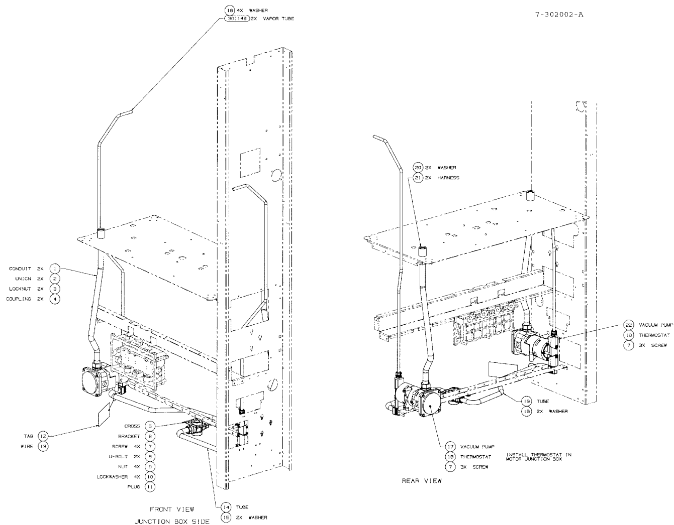
FIGURE 33. 7-302002-DWG - WAYNE VAC VAPOR RECOVERY MODULE
