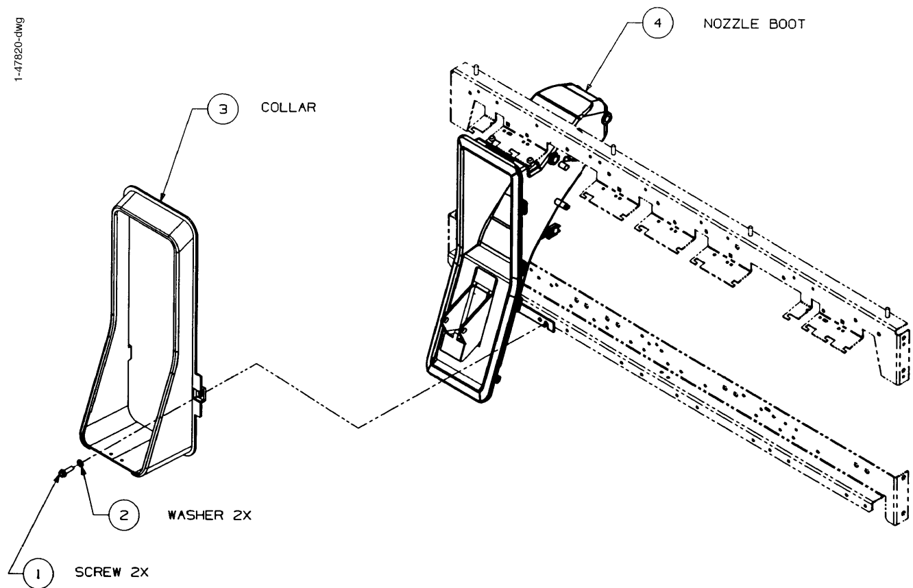
FIGURE 38. 1-47820-DWG - NOZZLE BOOT REMOTE
