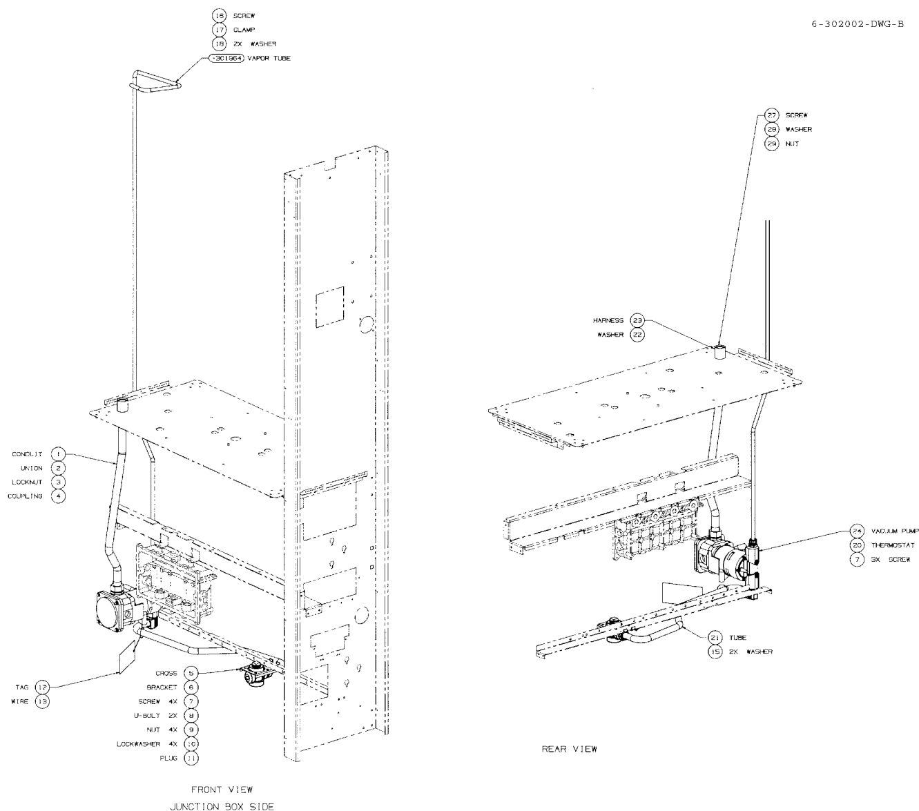
FIGURE 32. 6-302002-DWG - WAYNE VAC VAPOR RECOVERY MODULE
