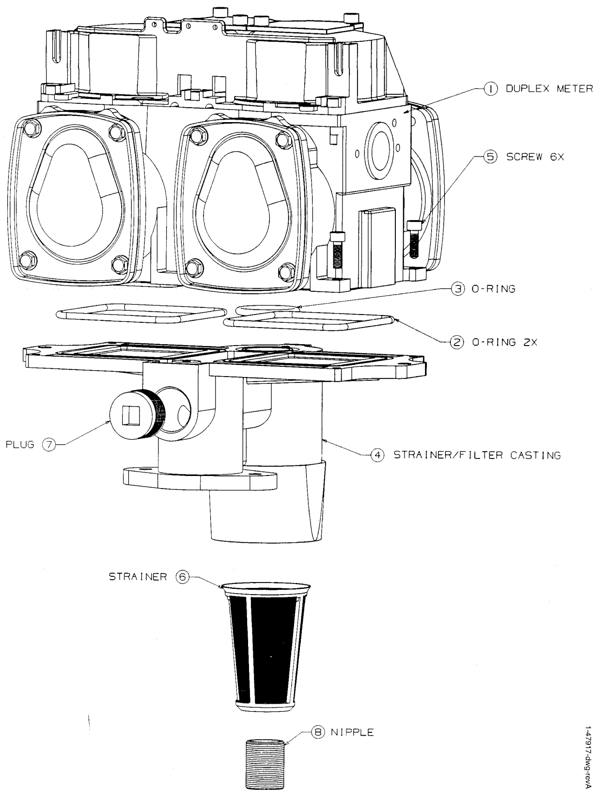
FIGURE 20. 1-47917-DWG - IMETER MODULE, REMOTE
