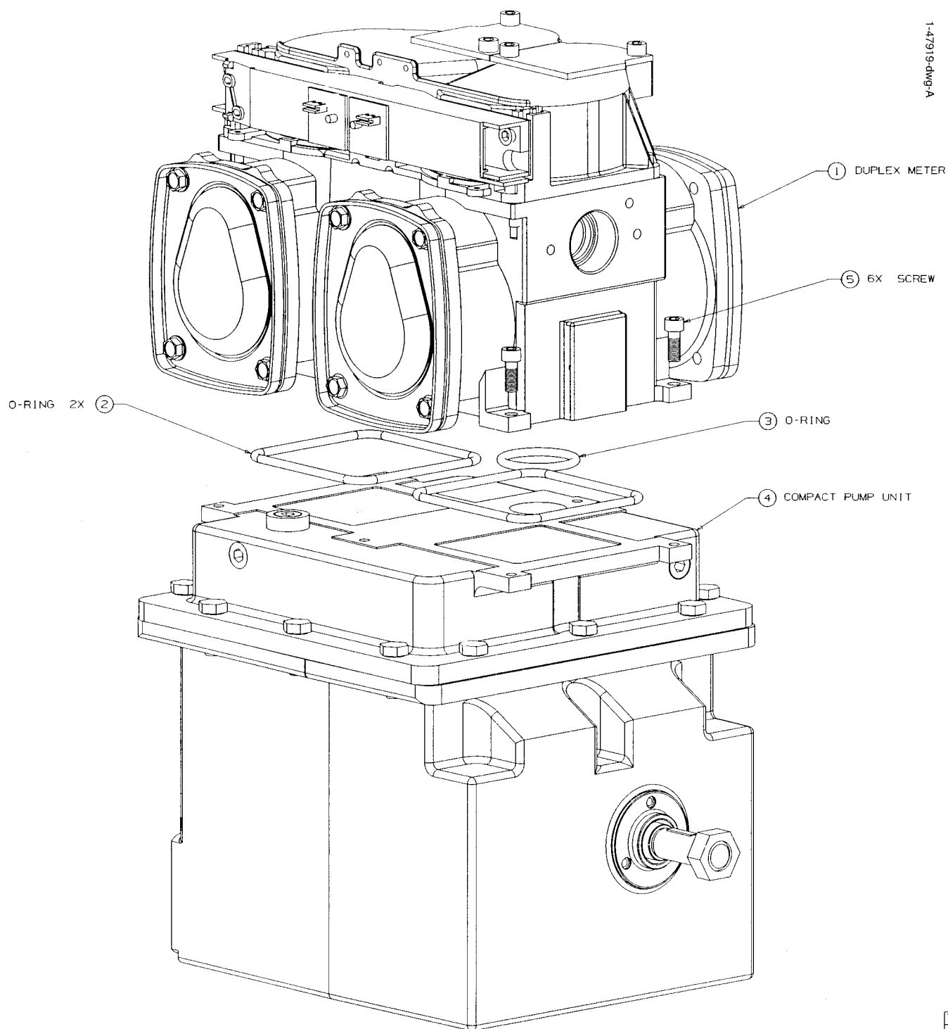
FIGURE 22. 1-47919-DWG - IMETER MODULE, 3/4 Suction
