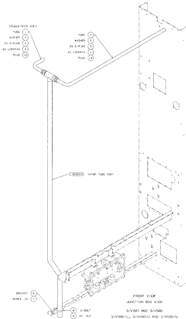
FIGURE 15. 1-302001-DWG - BALANCE VAPOR RECOVERY MODULE
