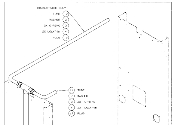
FRONT VIEW JUNCTION BOX SIDE 3/V595/U 3/V595 (NON-GASOLINE SEPARATE PRODUCT)
