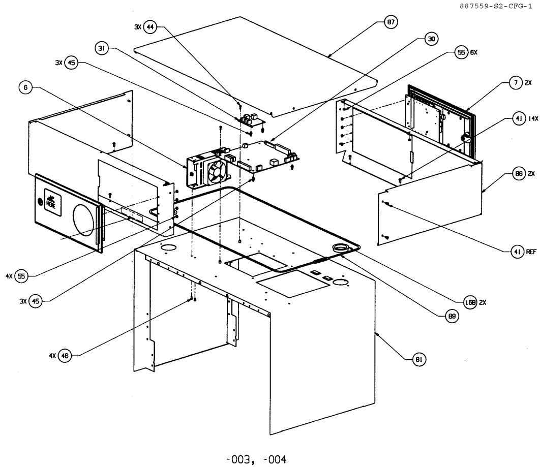
FIGURE 32. 887559-S2-CFG - WAYNE TRAC ENCLOSURE ASSY, 3/4 V NARROW
