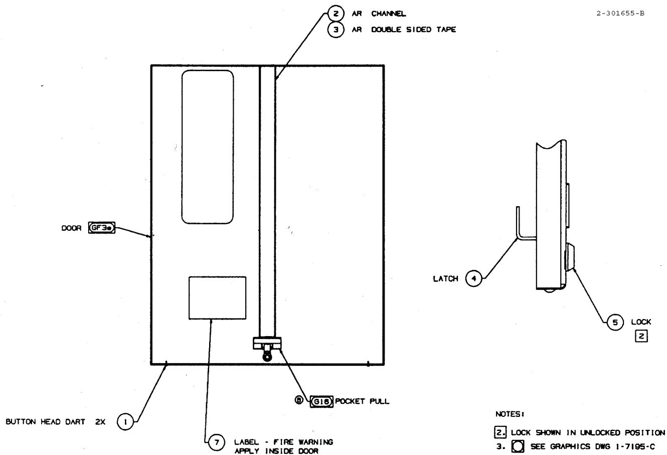
FIGURE 5. 2-301655-DWG - DOOR MODULE 3/V NARROW
