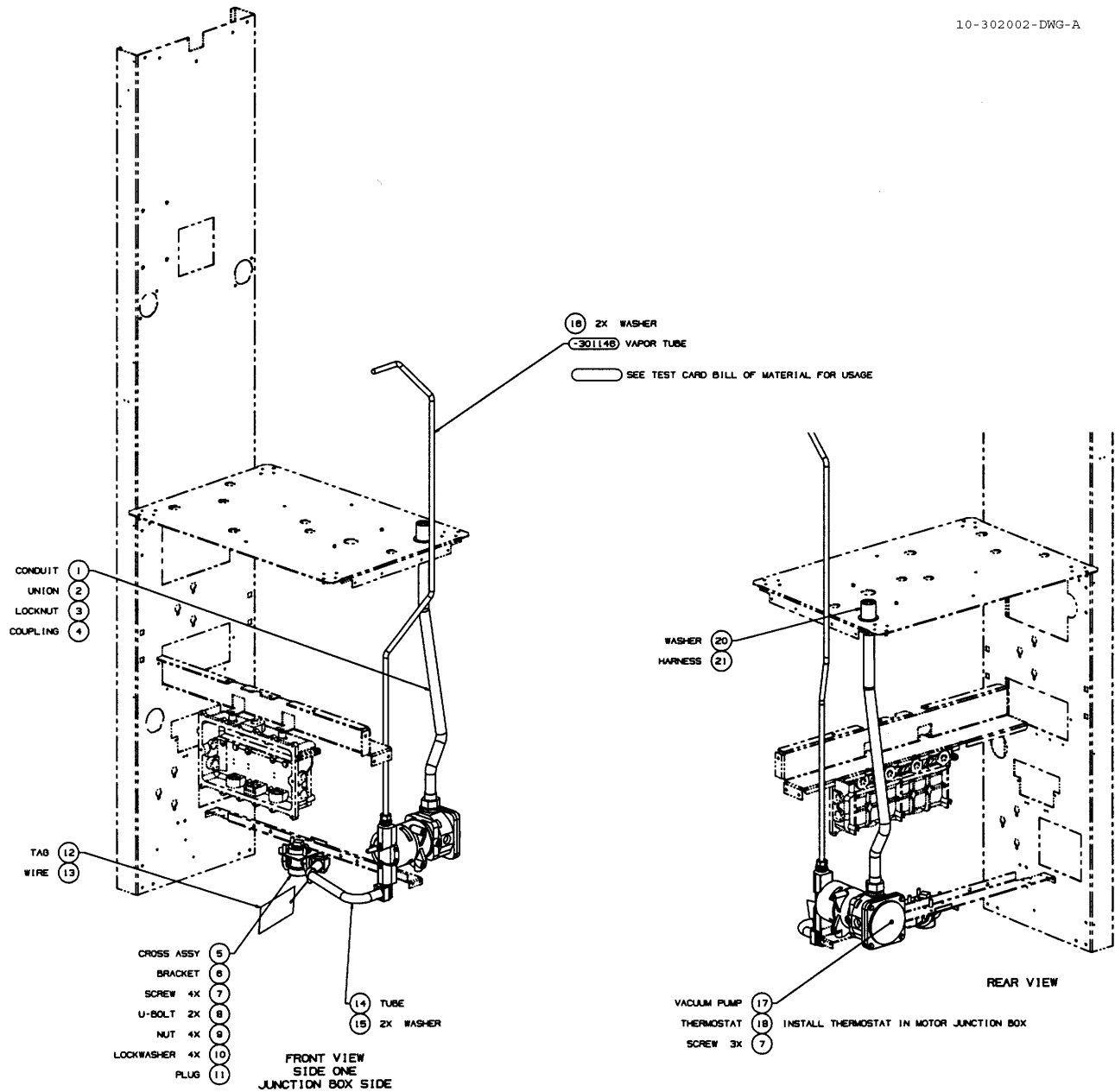
FIGURE 22. 10-302002 - WAYNE VAC VAPOR RECOVERY MODULE
