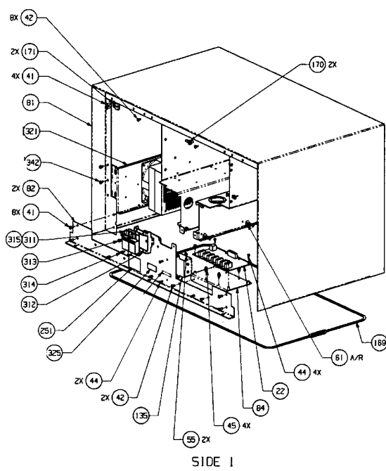
FIGURE 30. 887557-S2-CFG - ELECTRONIC HEAD MODULE 3/V NARROW
