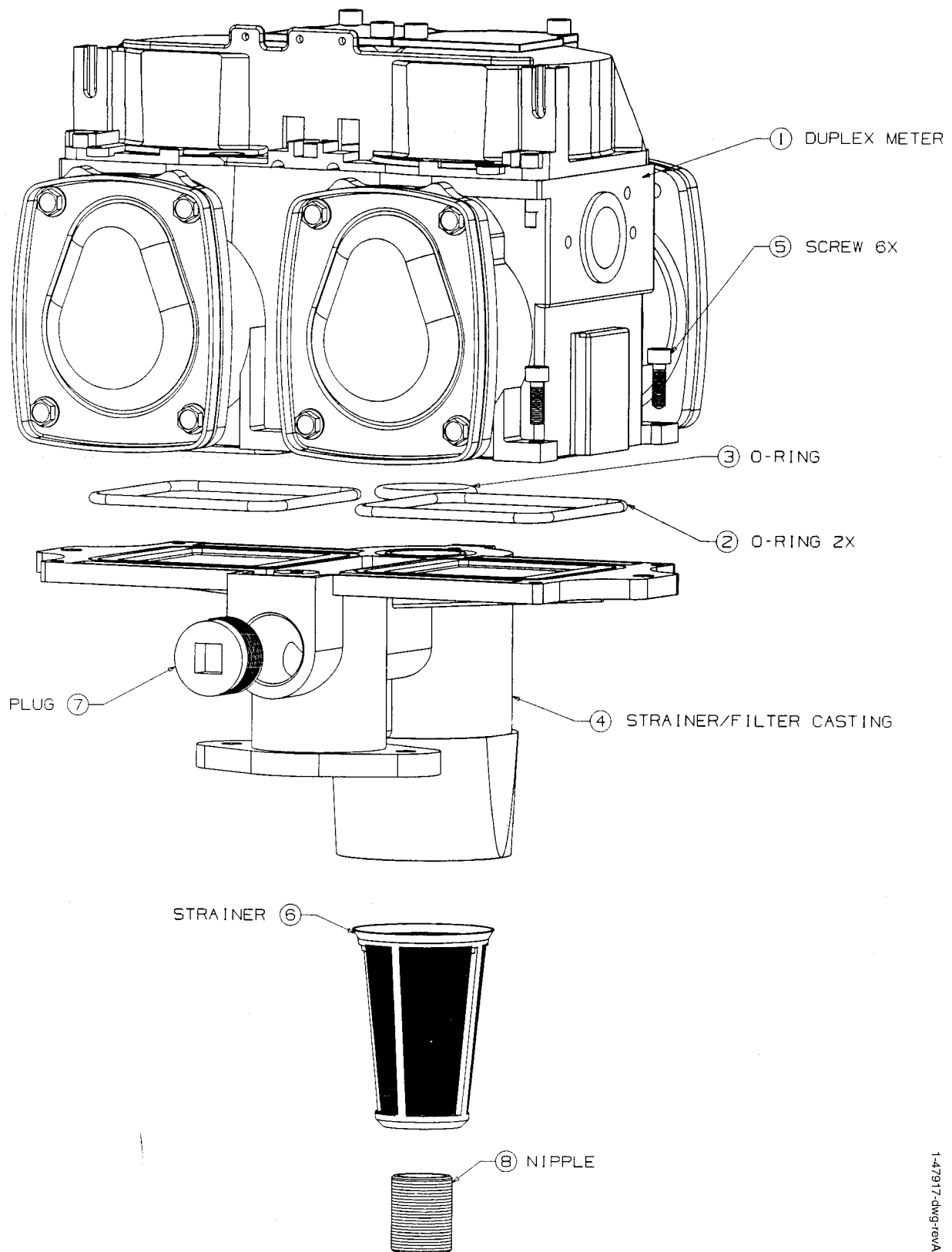
FIGURE 11. 1-47917-DWG - IMETER MODULE, REMOTE
