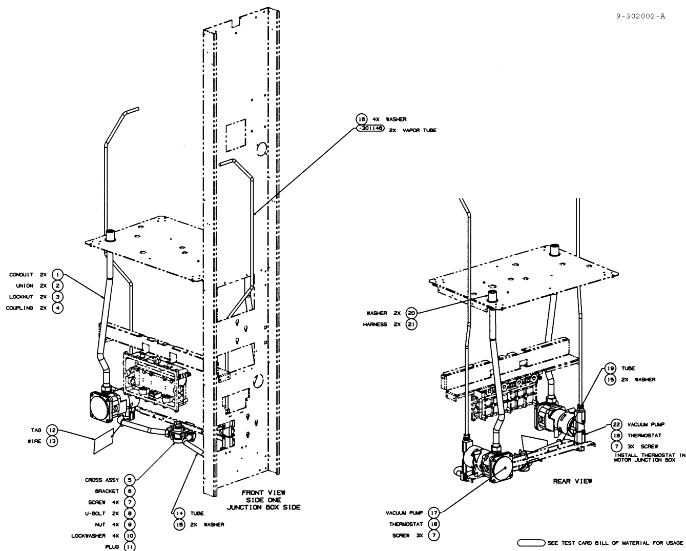
FIGURE 21. 9-302002-DWG - WAYNE VAC VAPOR RECOVERY MODULE
