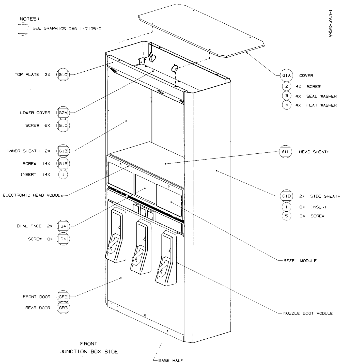
FIGURE 2. 1-47901-DWG - HOUSING MODULE
