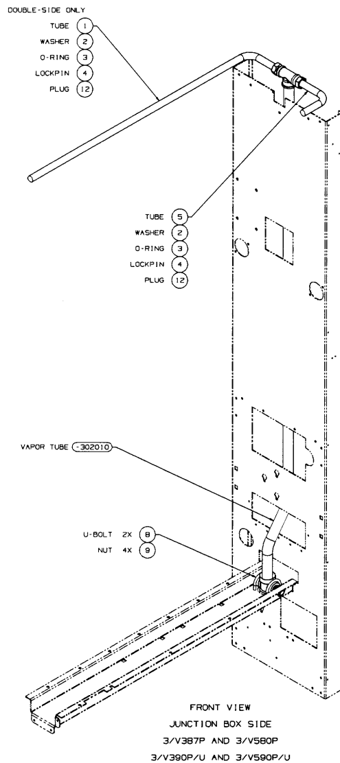
FIGURE 18. 13-302001-DWG - BALANCE VAPOR RECOVERY MODULE SUCTION
