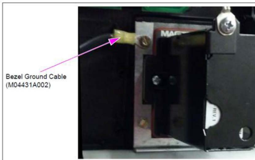
Figure 4: Bezel Ground Cable
