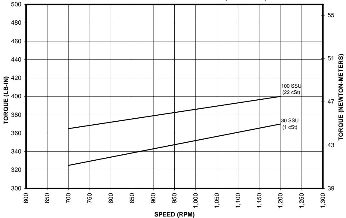
TORQUE REQUIRED AT 50 PSI (3.45 Bar)
