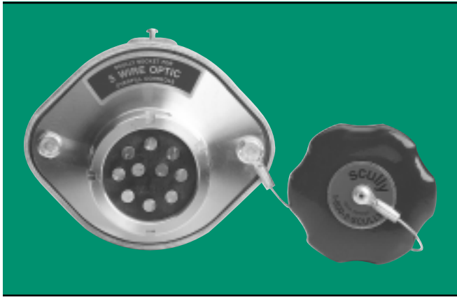
Scully Five-Wire Optic Socket with Polyvinyl Cap
